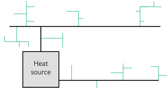
Fig. 06-1 Radial network
