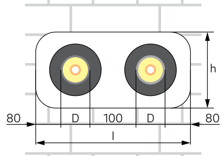
Fig. 05-5 Dimensions of wall penetration
