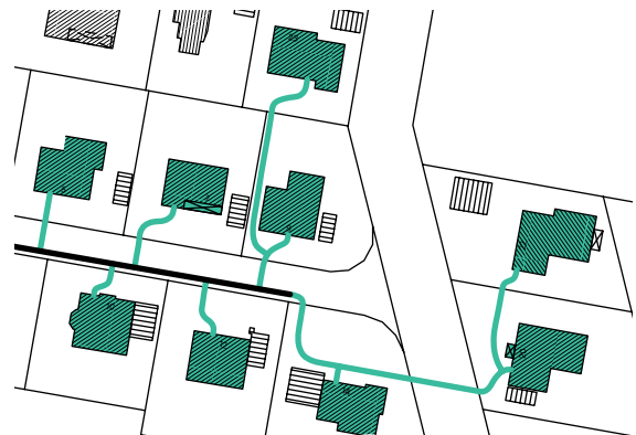
Fig. 06-6 Connecting different pipe systems
