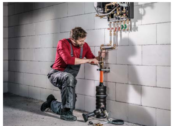
Fig. 05-2 Transfer point
