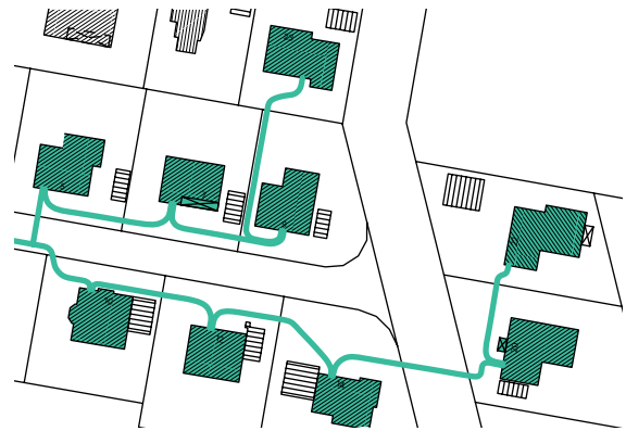
Fig. 06-5 House-to-house line arrangement/ building-to-building piping
