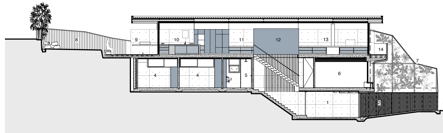
Section AA
