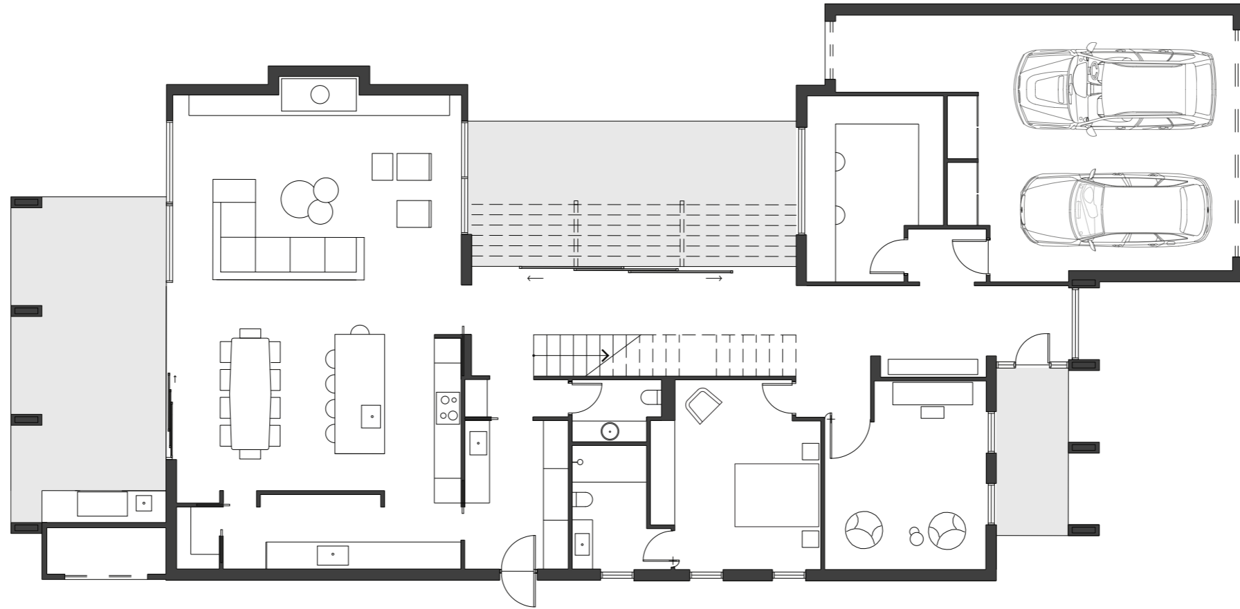
GROUND FLOOR PLAN 0 5m
