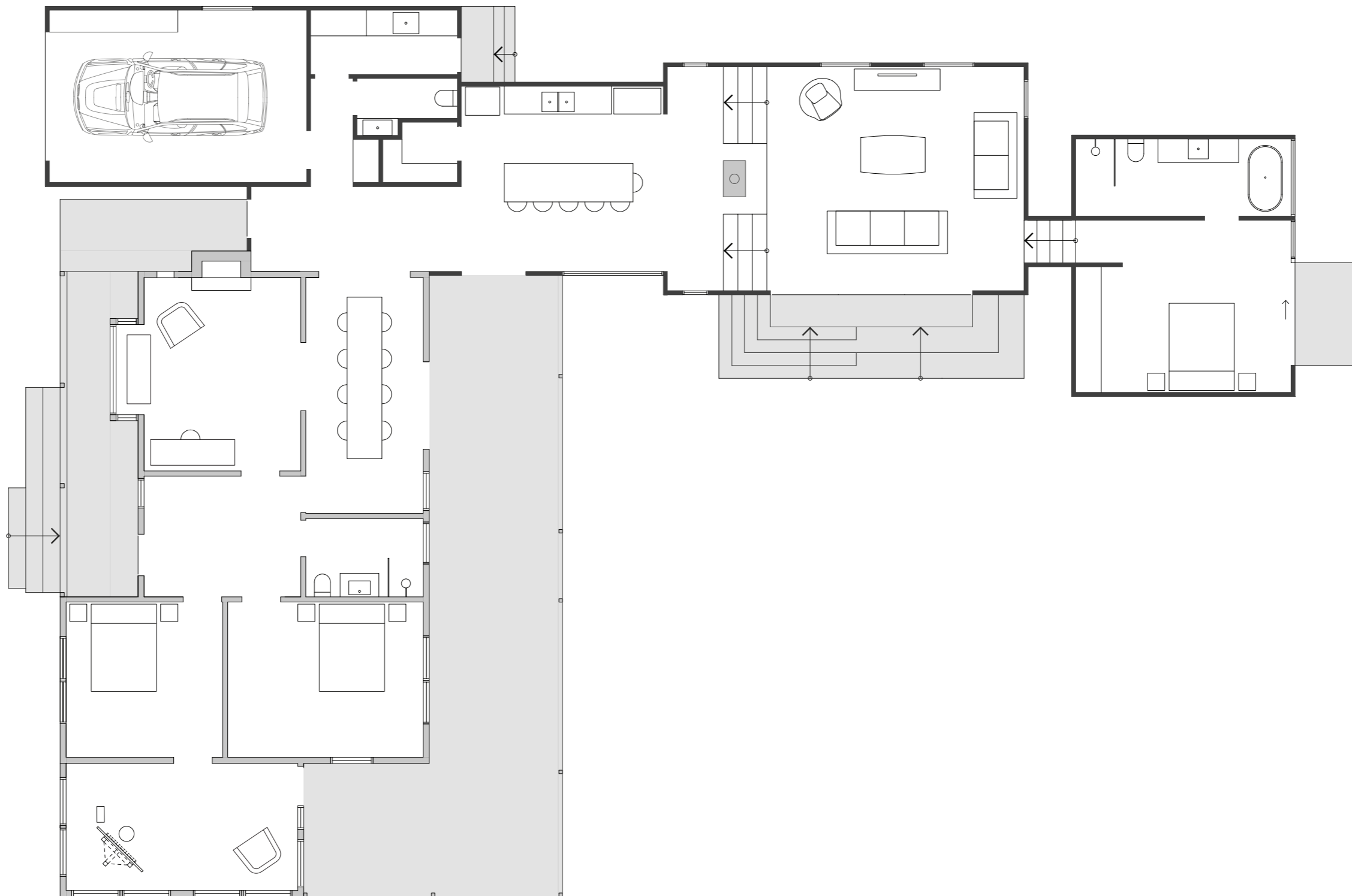
GROUND FLOOR PLAN 0 5m
