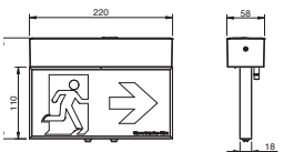
CEILING MOUNT (SURFACE)
