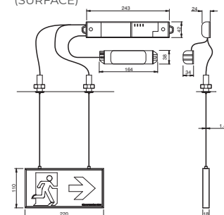
CEILING MOUNT CABLE SUSPENDED (SURFACE)
