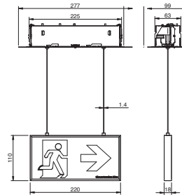
CEILING MOUNT CABLE SUSPENDED (RECESSED)
