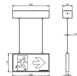
CEILING MOUNT ROD SUSPENDED (SURFACE)
