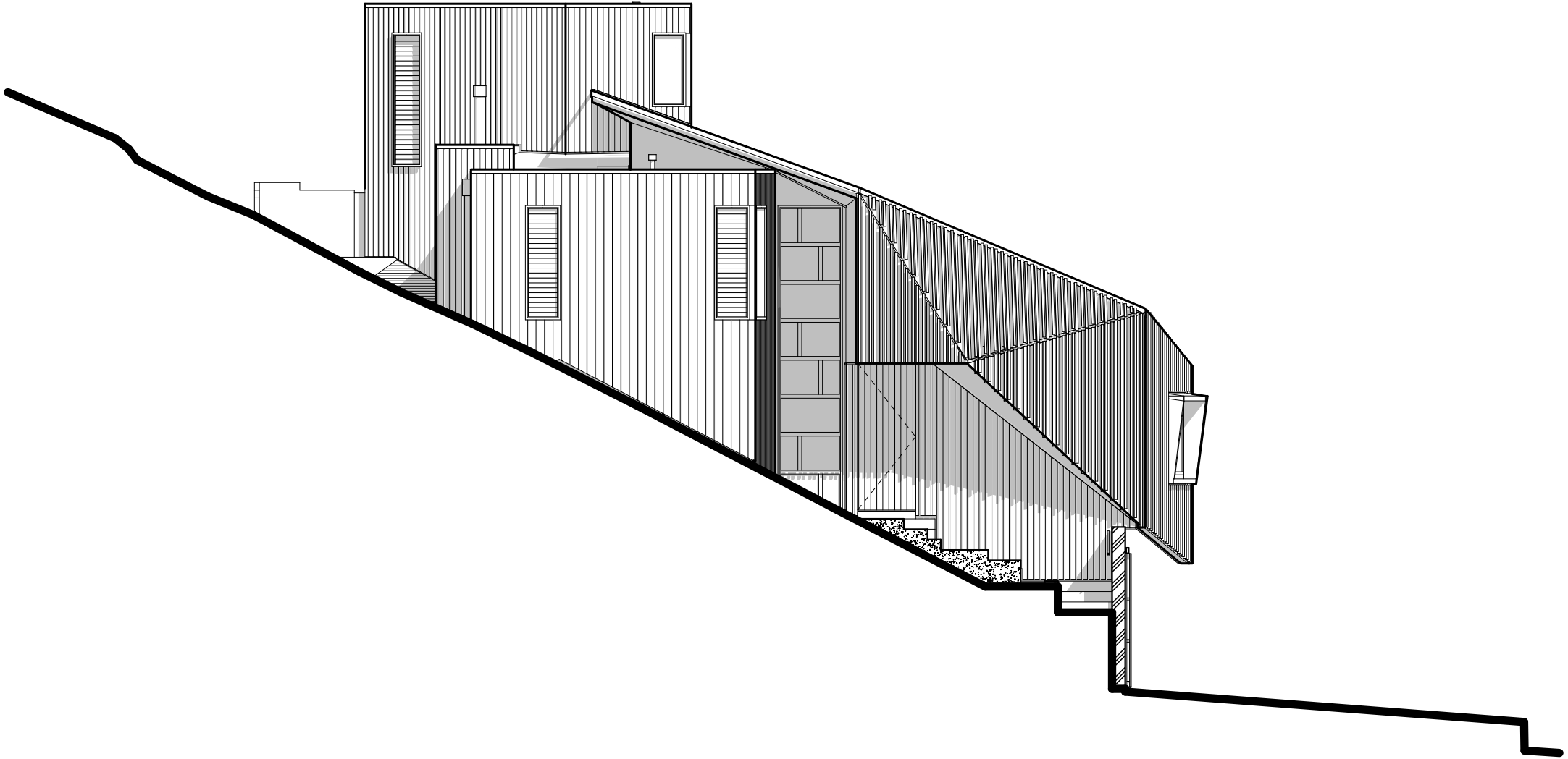
WEST ELEVATION
