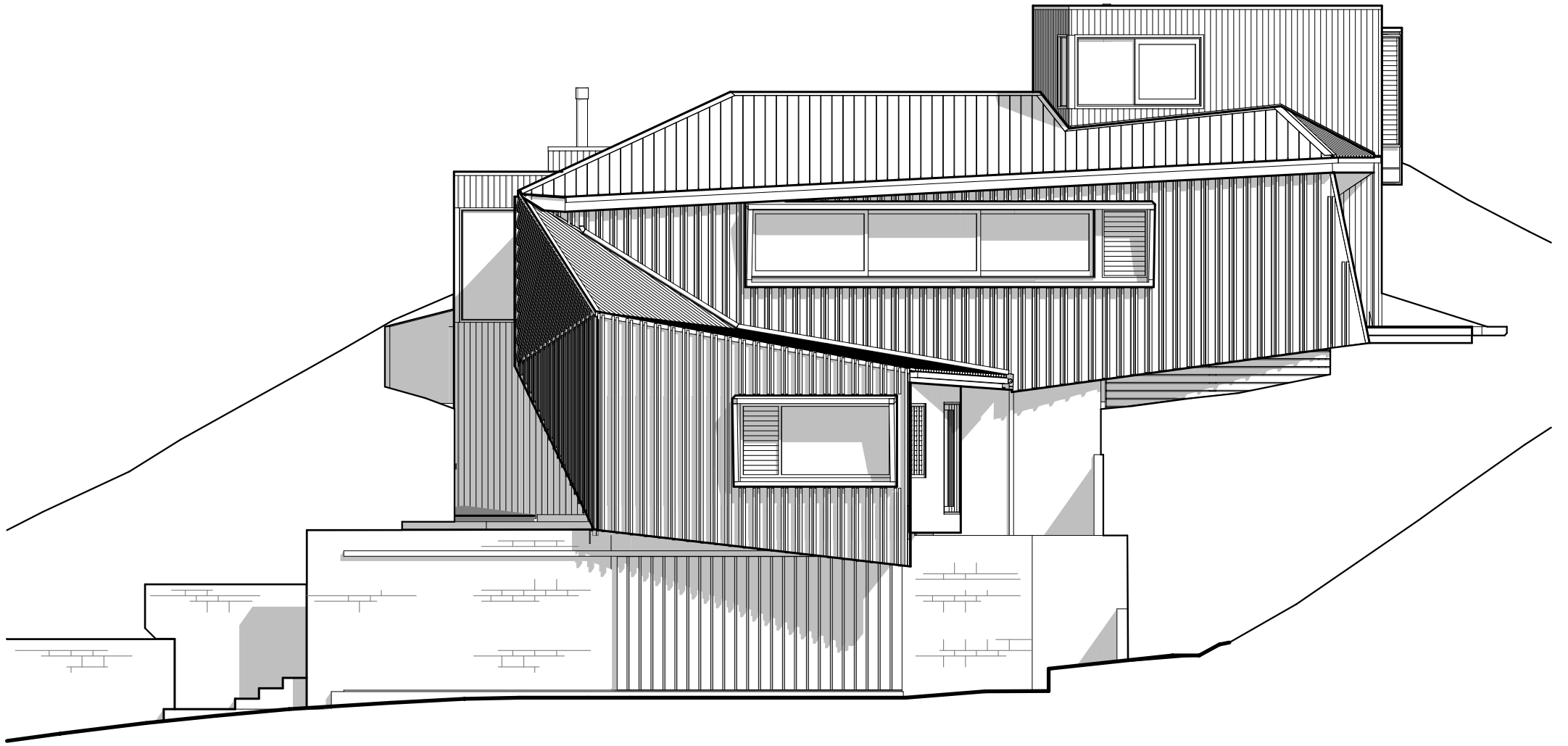
SOUTH ELEVATION
