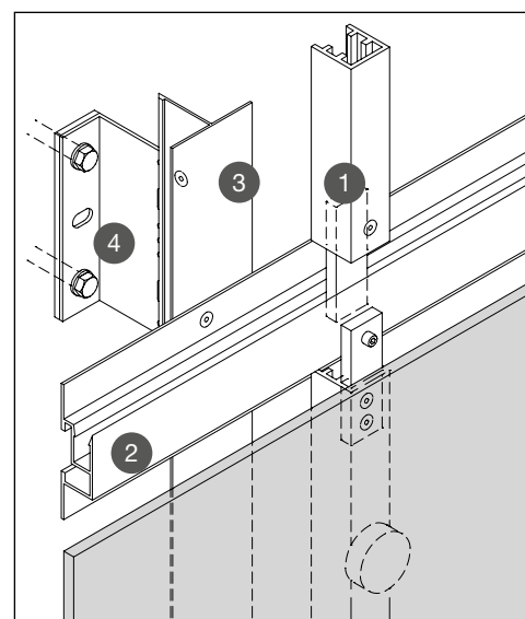
KerAion® Quadro fastening with bearing profile
