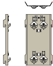
Article 700 OmegaV, painted*, RAL 7021 Material: AlMg3 H22 (EN AW-5754) painted black, for installation with joint spacer K20/8
