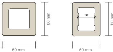
Cross-section of rectangular tube
