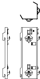
Article 705 OmegaV, external angle, bright* Material: AlMg3 H22 (EN AW-5754) unpainted, for the installation of mitre-cut panels and external angle profiles
