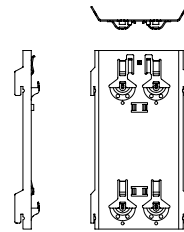
Article 701 OmegaV, bright* Material: AlMg3 H22 (EN AW-5754) unpainted, for installation with joint profile Single K20/8
