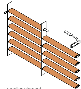
Lamellar element
