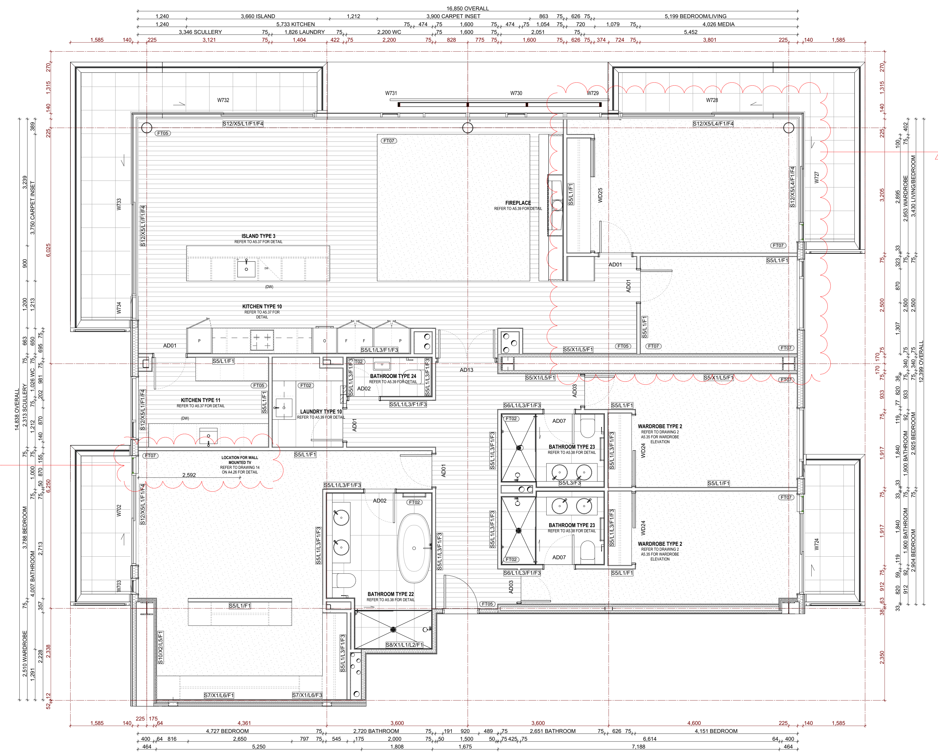
FLOOR PLAN SCALE 1:50
