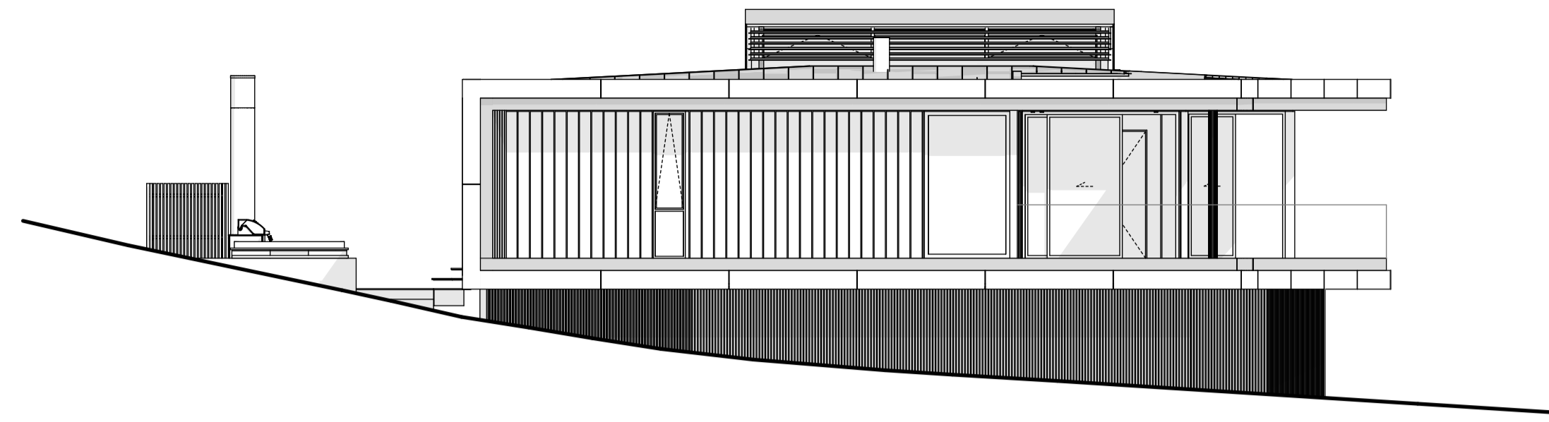
North Elevation
