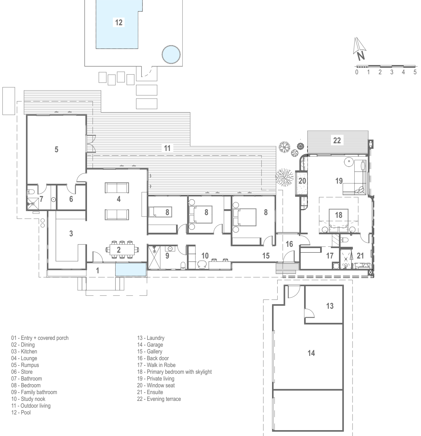
FLOOR PLAN : COMPLETE
