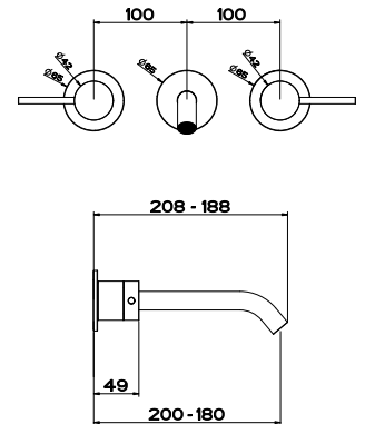
45089+54094 THREE HOLE WALL MIXER
