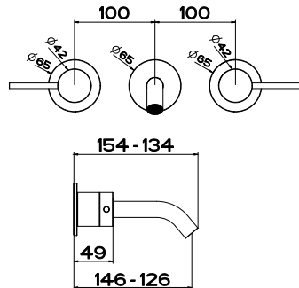
45089+54092 THREE HOLE WALL MIXER
