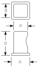
HB 2360 Knob
