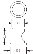
HB 2260 Knob
