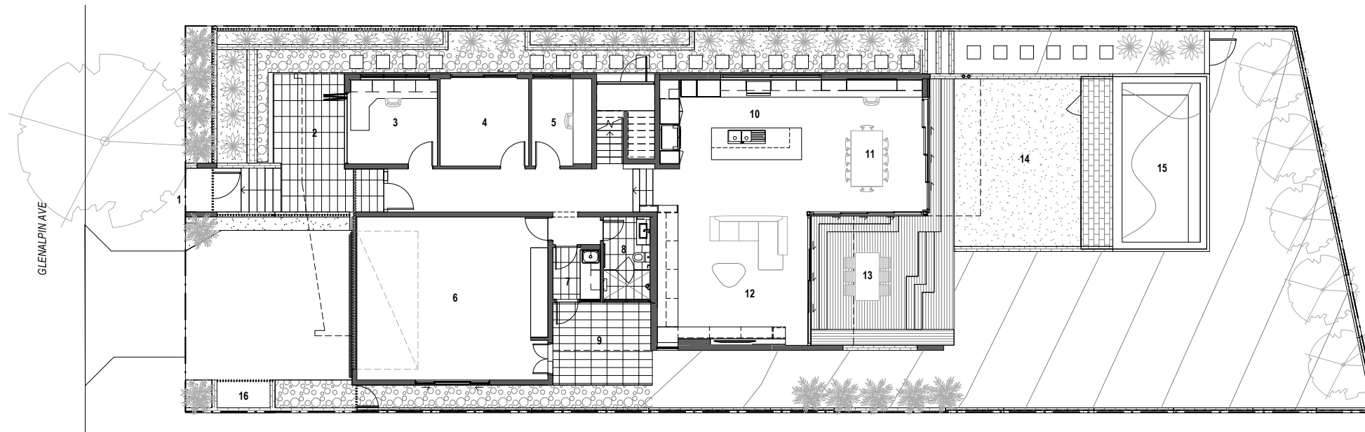
1 Gatehouse | 2 Courtyard | 3 Office | 4 Gym | 5 Hobby | 6 Garage | 7 Laundry | 8 Bathroom | 9 Drying | 10 Kitchen | 11 Dining | 12 Living | 13 Deck | 14 Lawn | 15 Pool | 16 Bins
