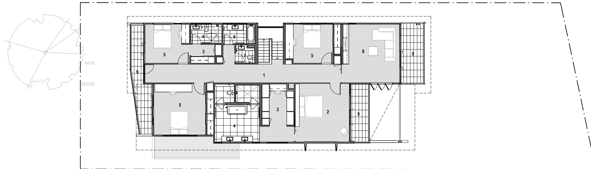
1 Breezeway | 2 Master bedroom | 3 Walk in robe | 4 Ensuite | 5 Bedroom | 6 Bathroom | 7 Powder room | 8 Lounge | 9 Balcony
