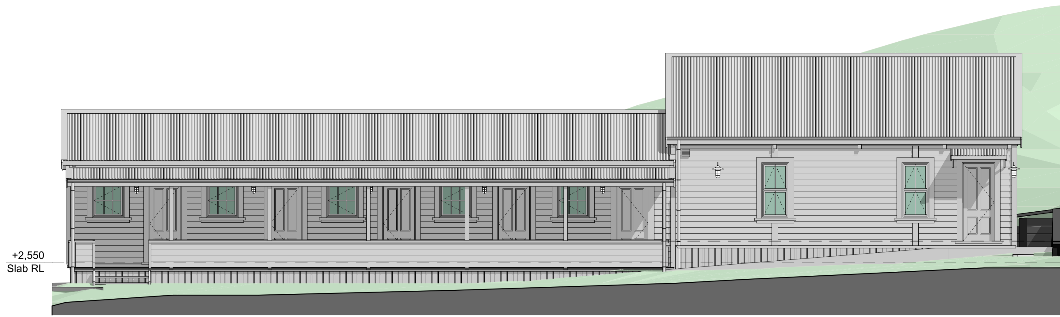
North Elevation
