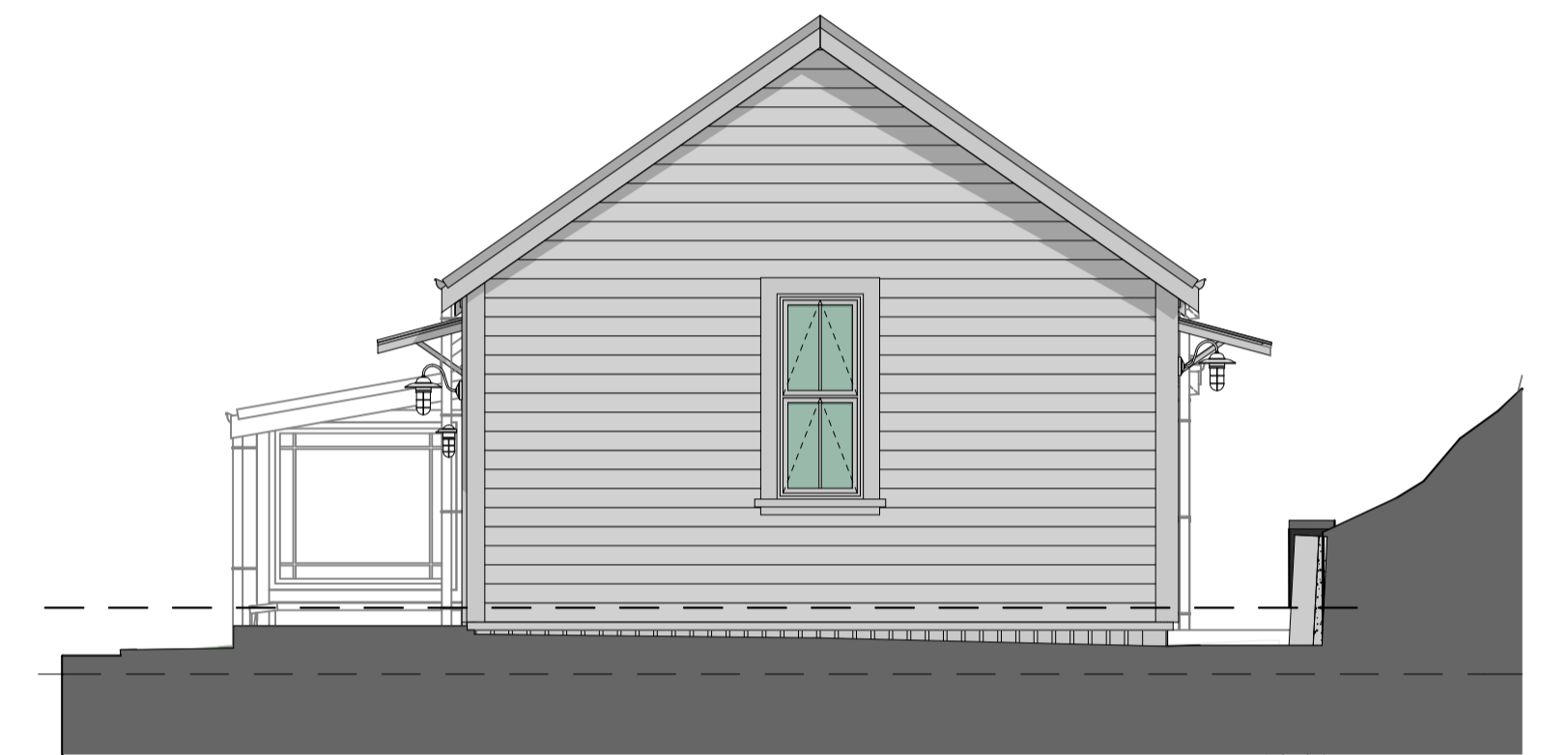
West Elevation
