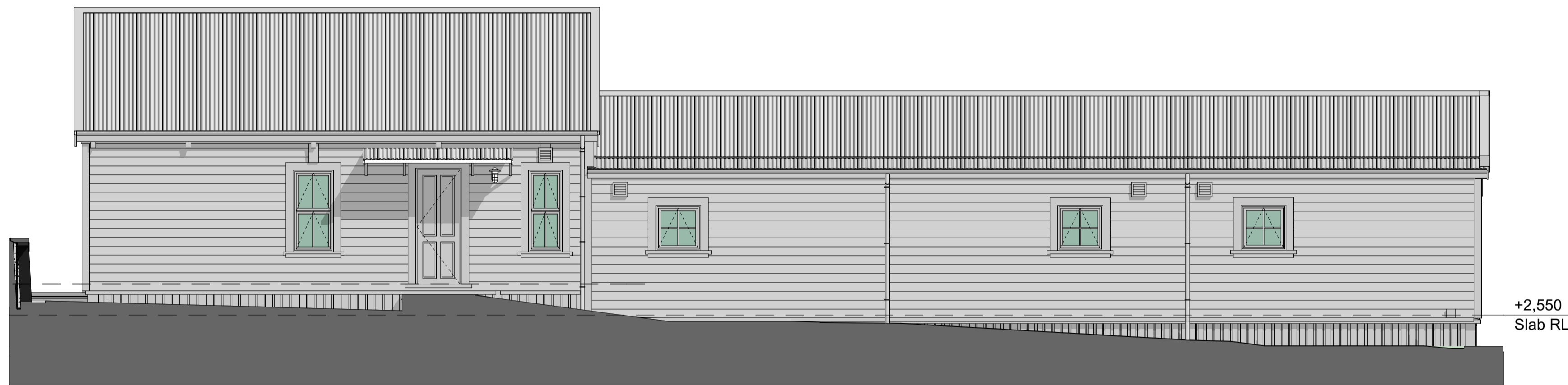
South Elevation
