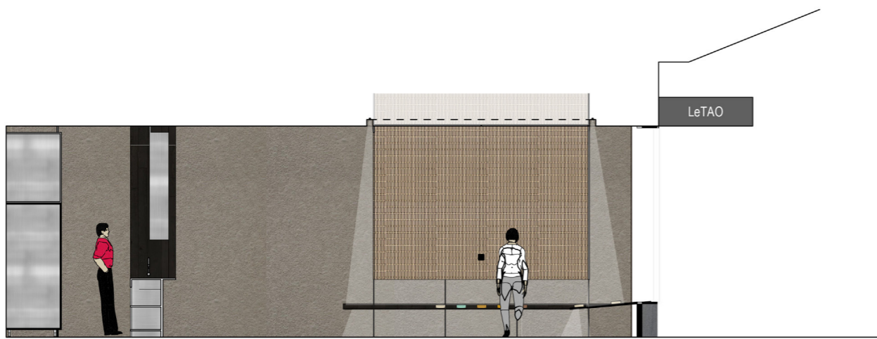
INTERIOR ELEVATION C
