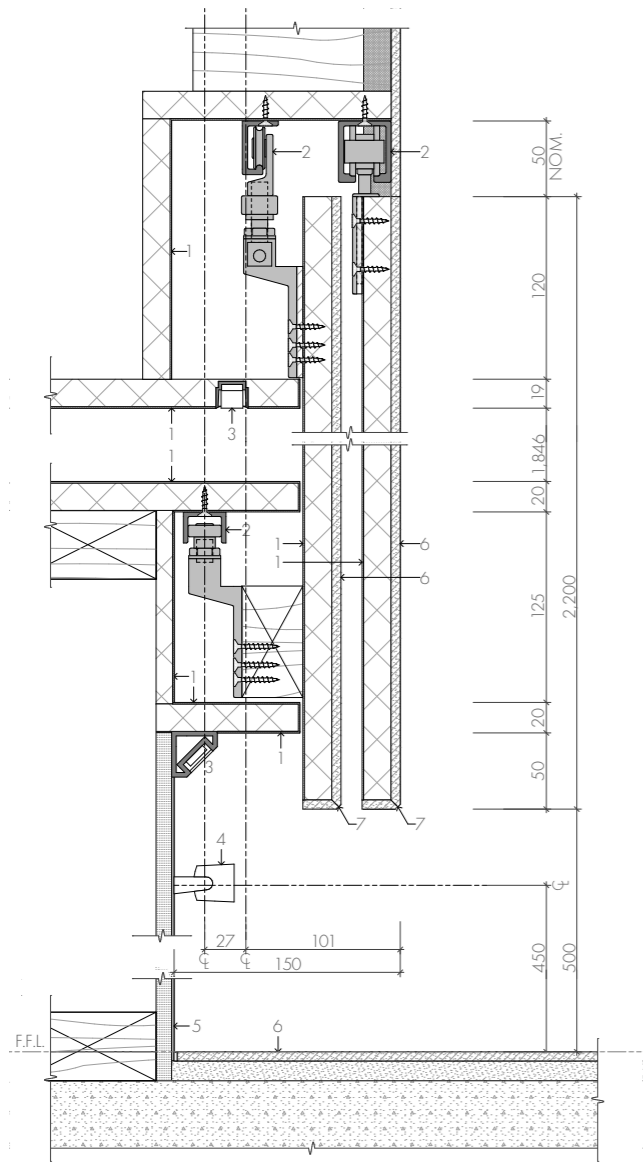
DETAIL SECTION - sliding walls
