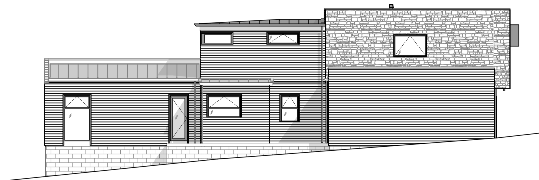
East Elevation
