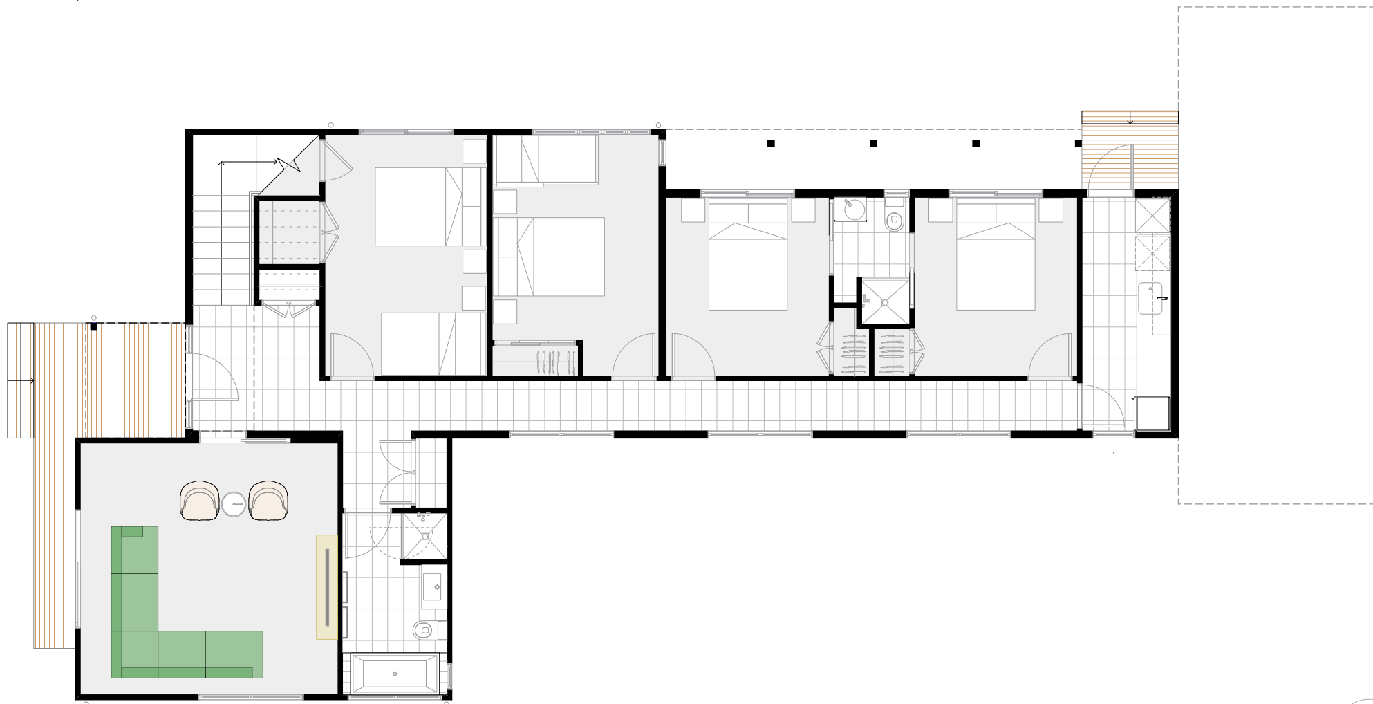
THE OWLS RETREAT - LAKE OKAREKA - FLOOR PLAN - 1:50
