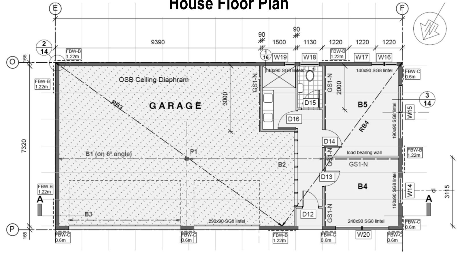
Garage Floor Plan
