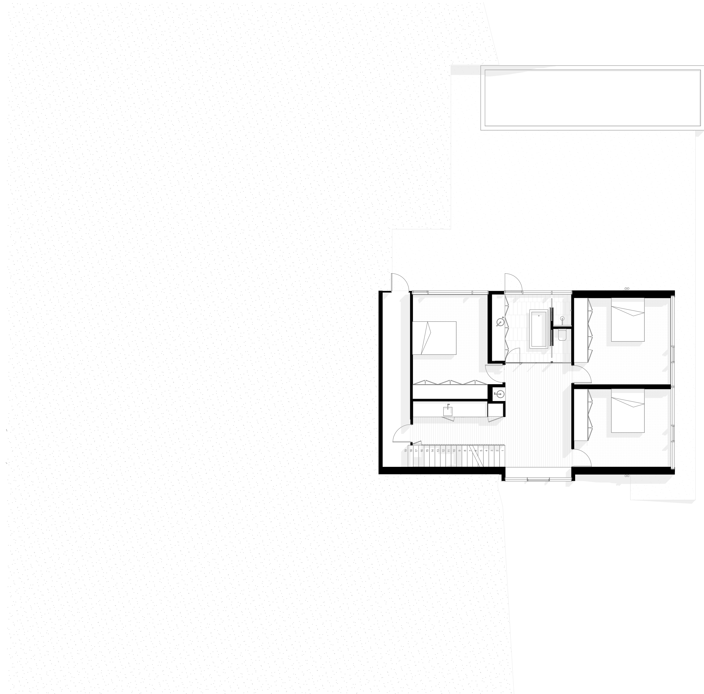
1:100 | LOWER FLOOR PLAN
