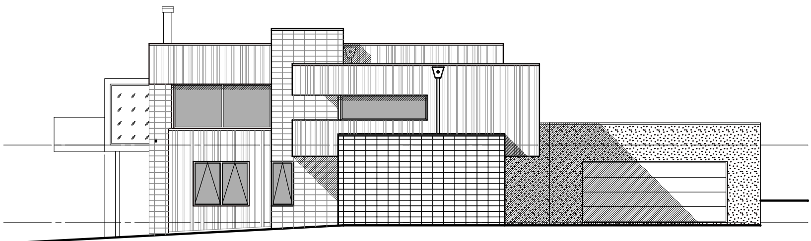
west elevation
