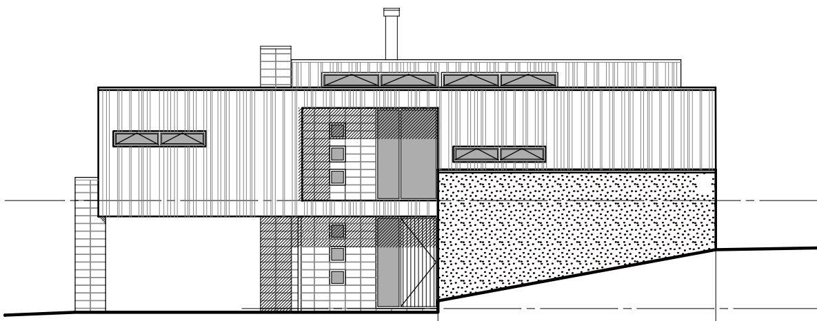
south elevation
