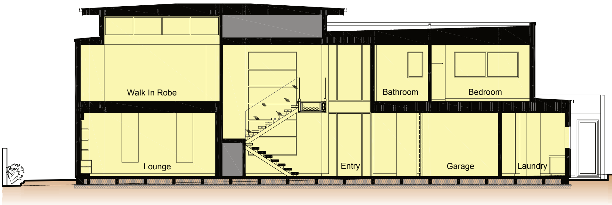
cross section
