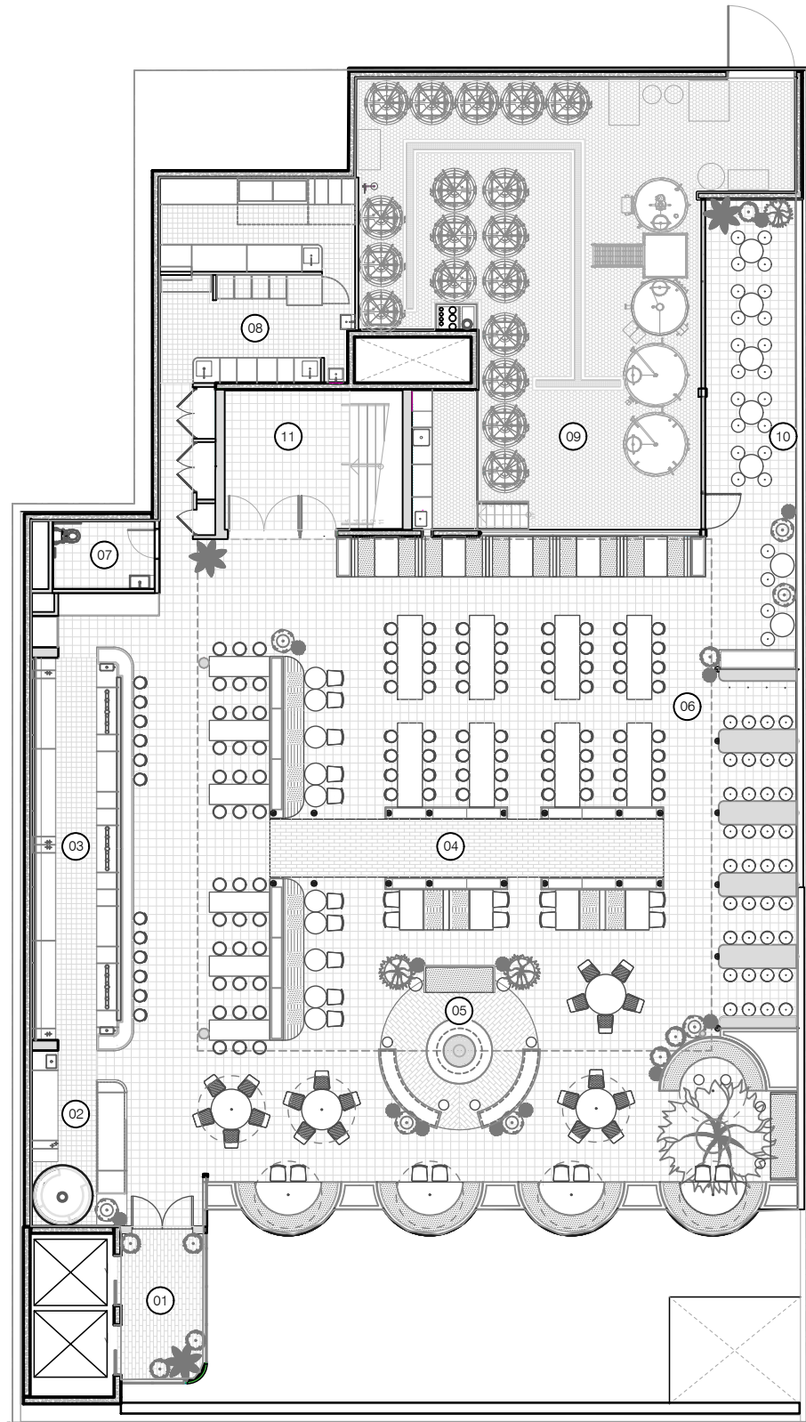
ROOFTOP LEVEL
