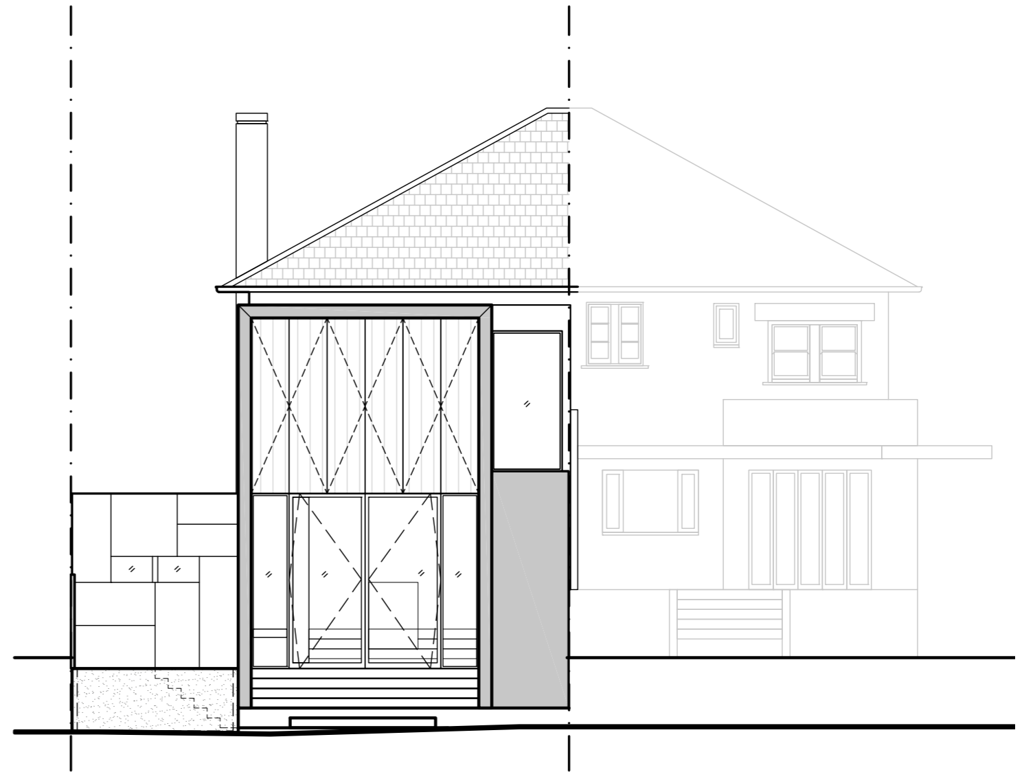
Rear Elevation
